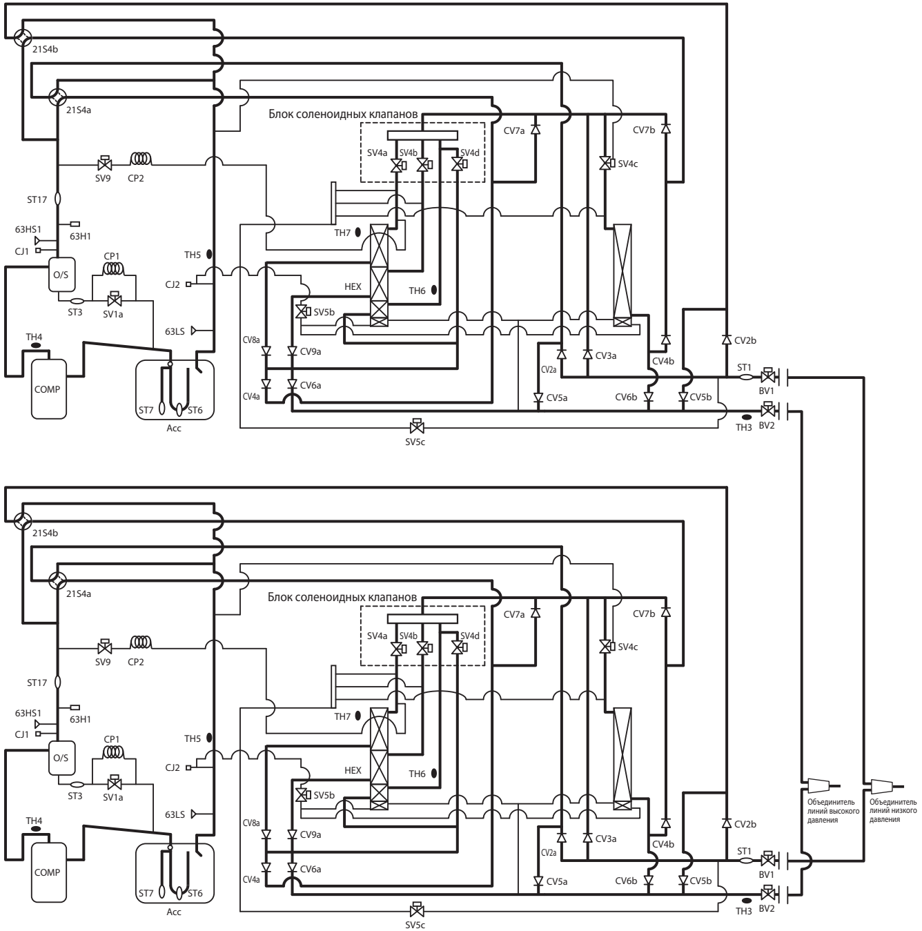
(13) PURY-P900YSJM-A(-BS), PURY-EP700YSJM-A(-BS)
