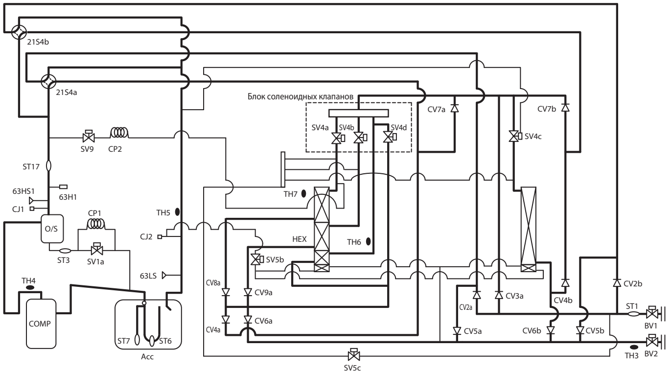
(8) PURY-P450YJM-A(-BS), PURY-EP350YJM-A(-BS)
